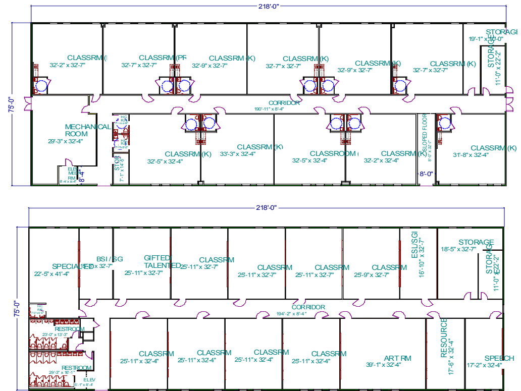
whitley CR-19130c; SECOND FLOOR 16301 sq ft
