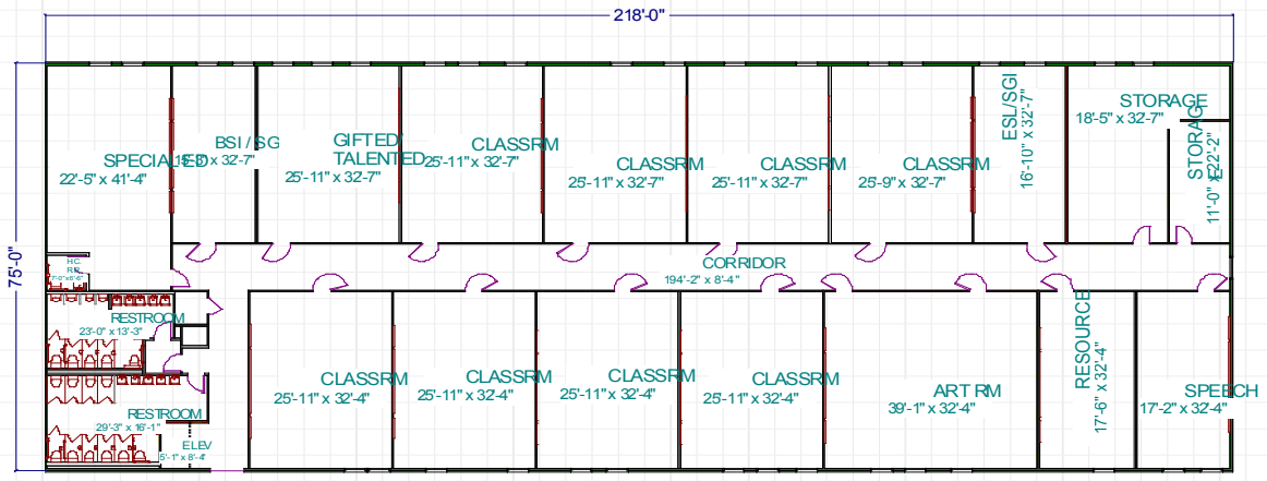
SECOND FLOOR
