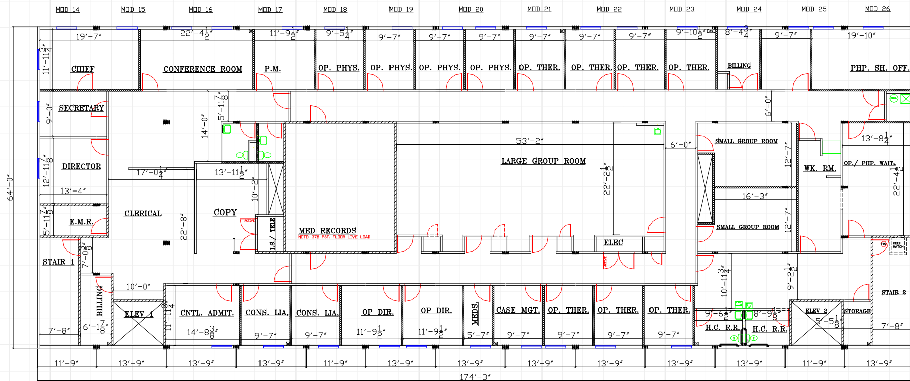
SECOND FLOOR
