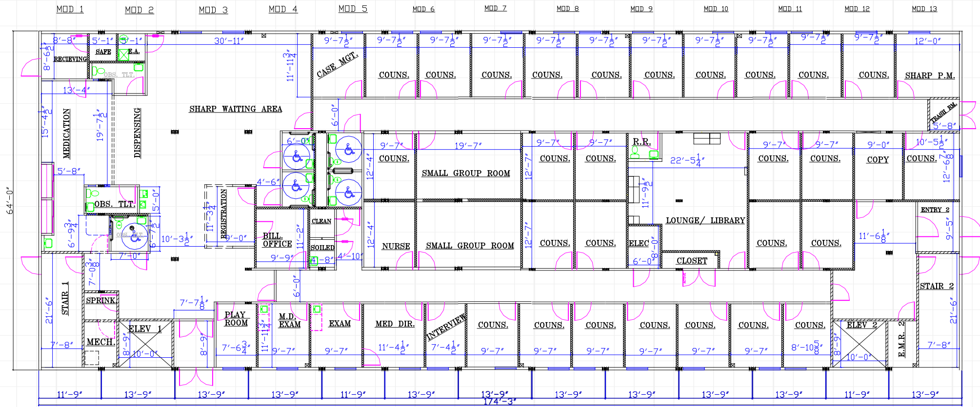
FIRST FLOOR
