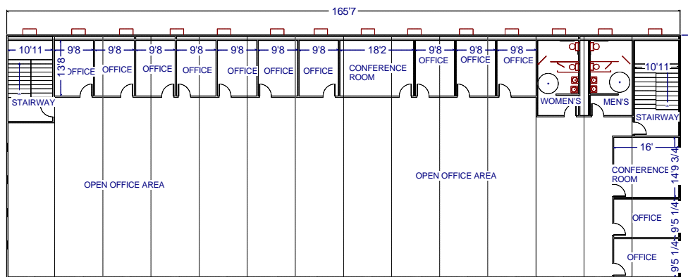
whitley MB-12344-2 (OPTION #2) SECOND FLOOR
