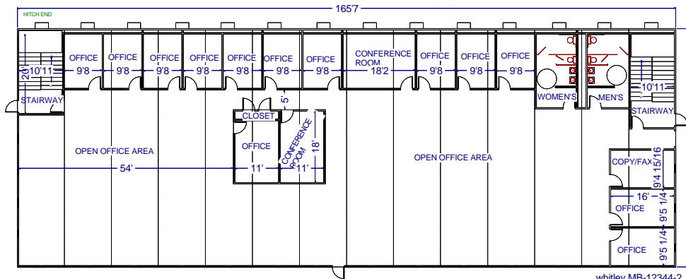
whitley MB-12344-2 (OPTION #2) FIRST FLOOR
