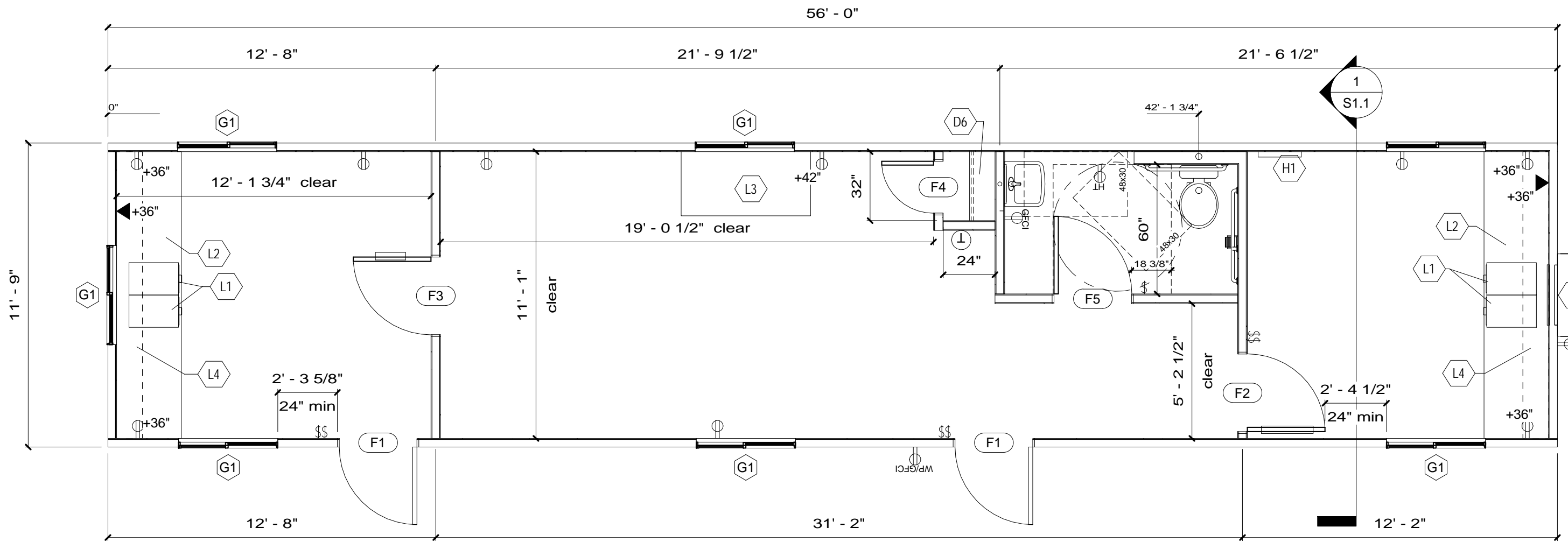
1 Floor Plan 1/4" = 1'-0"
