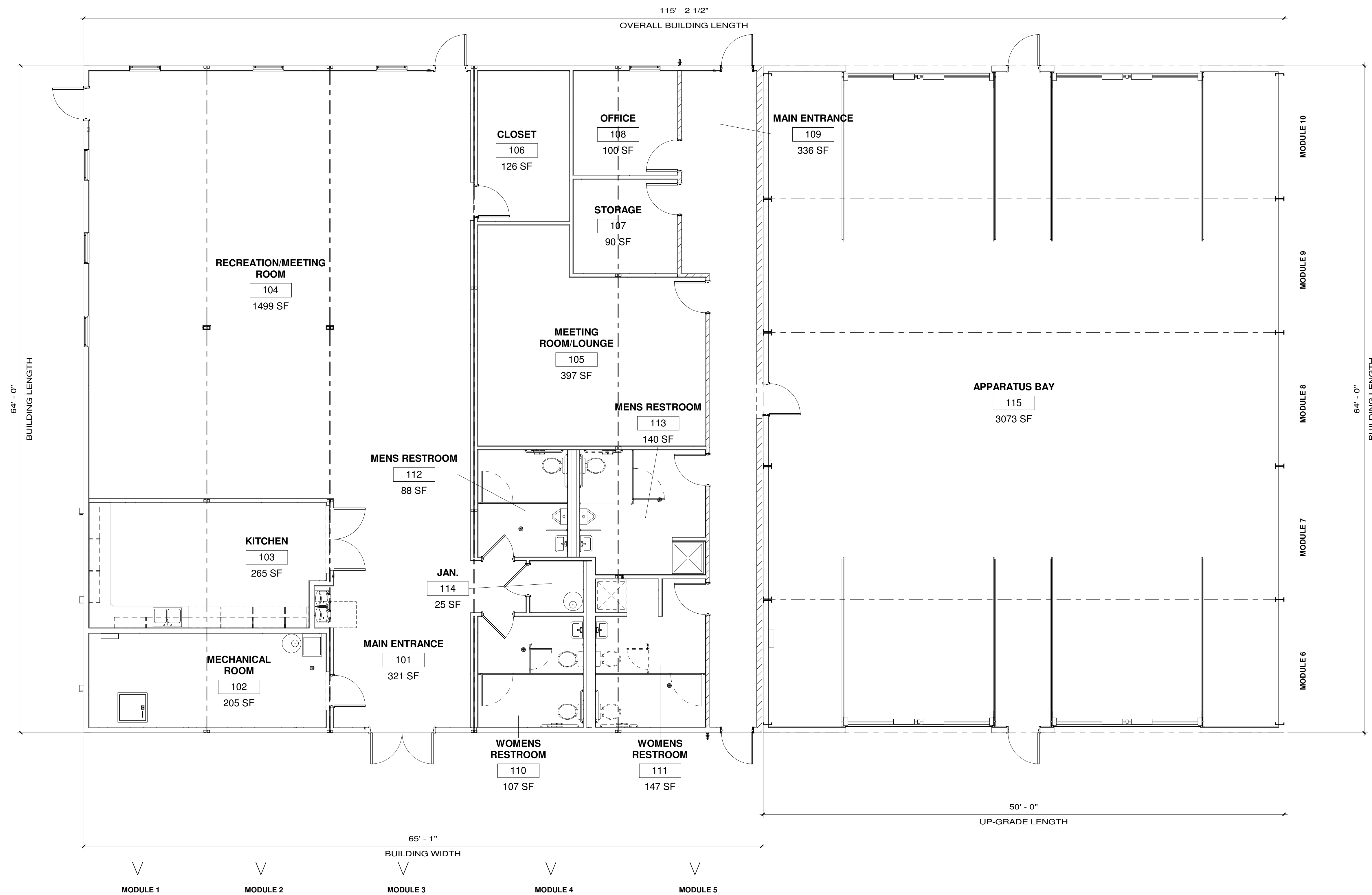
1 Floor Plan 3/16" = 1'-0"
